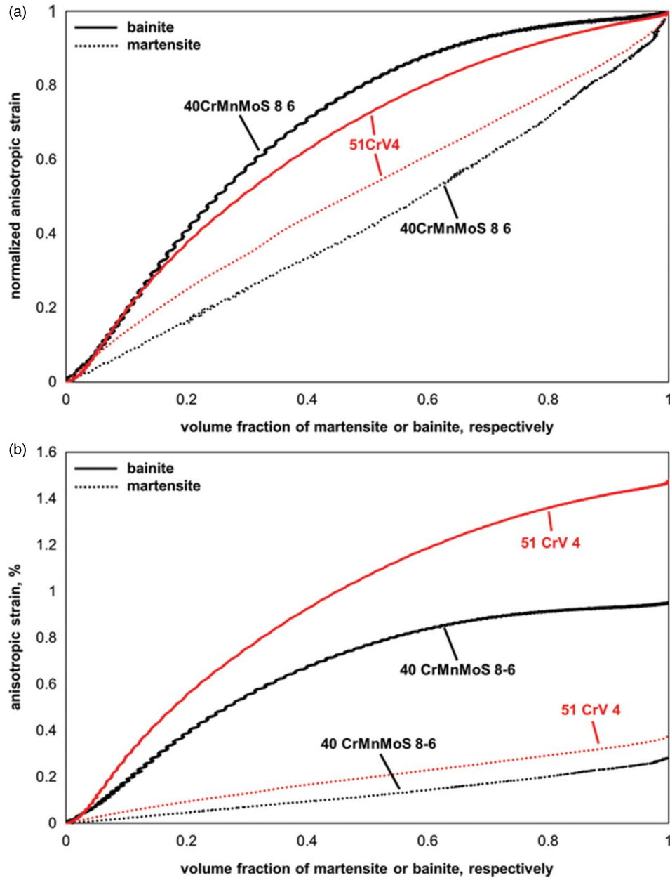
Figure 1. Evolution of anisotropic strain with volume fraction of martensite and bainite presented in (a) normalized and (b) absolute fashion for a martensitic and an isothermal bainitic phase transformation at 340°C under 100 MPa superimposed stress. The phase transformations followed an austenitization treatment at 1200°C for 10 s for both materials.
