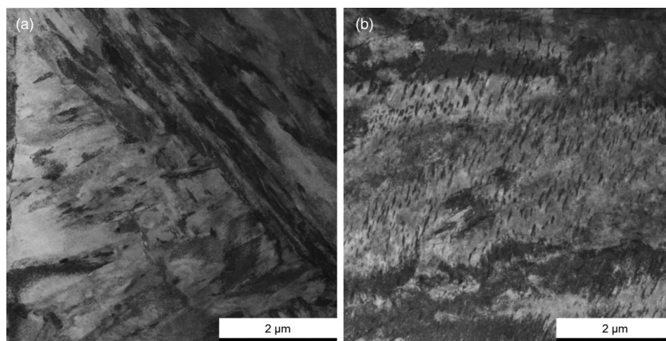
Figure 2. TEM images illustrating the microstructure upon (a) austenite-to-martensite and (b) austenite-to-bainite phase transformations under 100 MPa superimposed stress in a low-alloy 40 CrMnMoS 8-6 tool steel.
